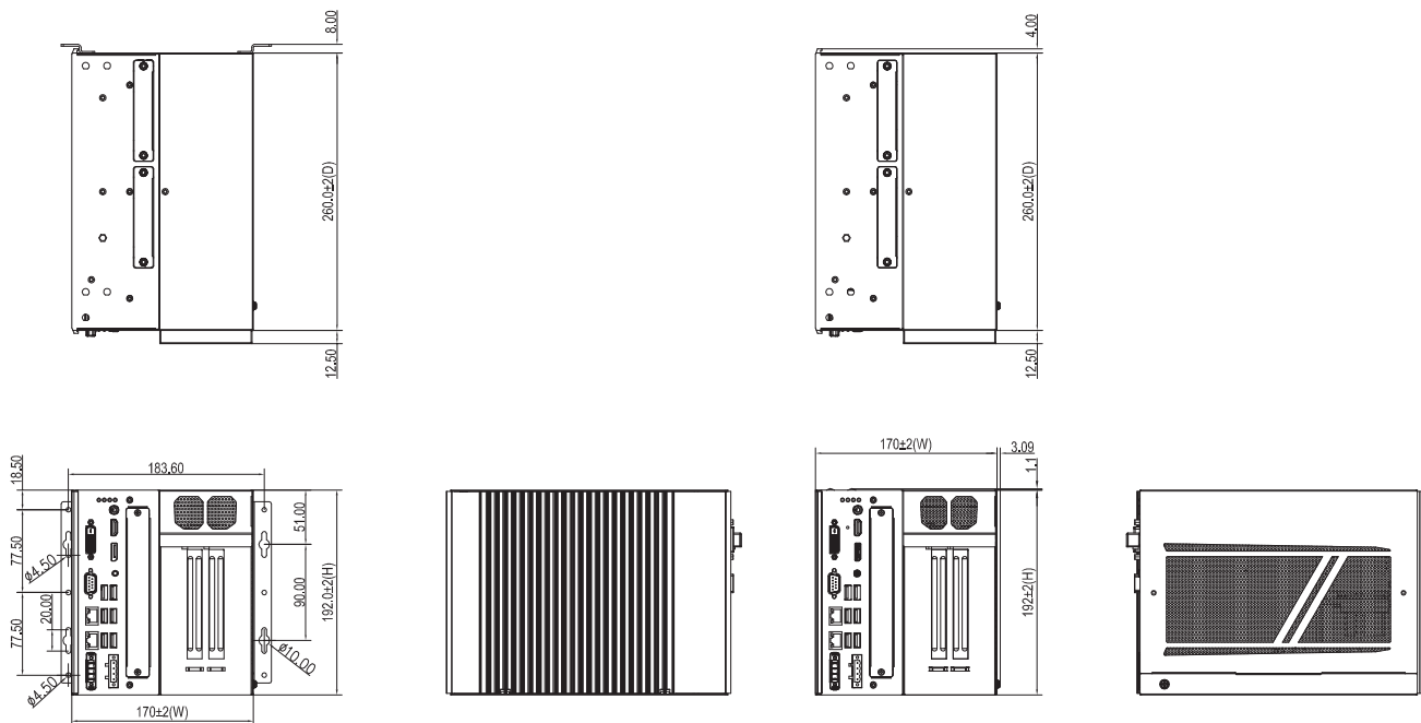
Option-wall mount
