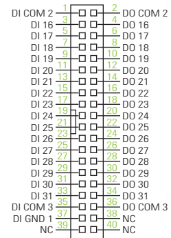
40-pin Box-Header (CN2) AX92351-64CH only
