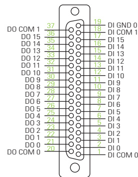
37-pin Female Connector (CN1)
