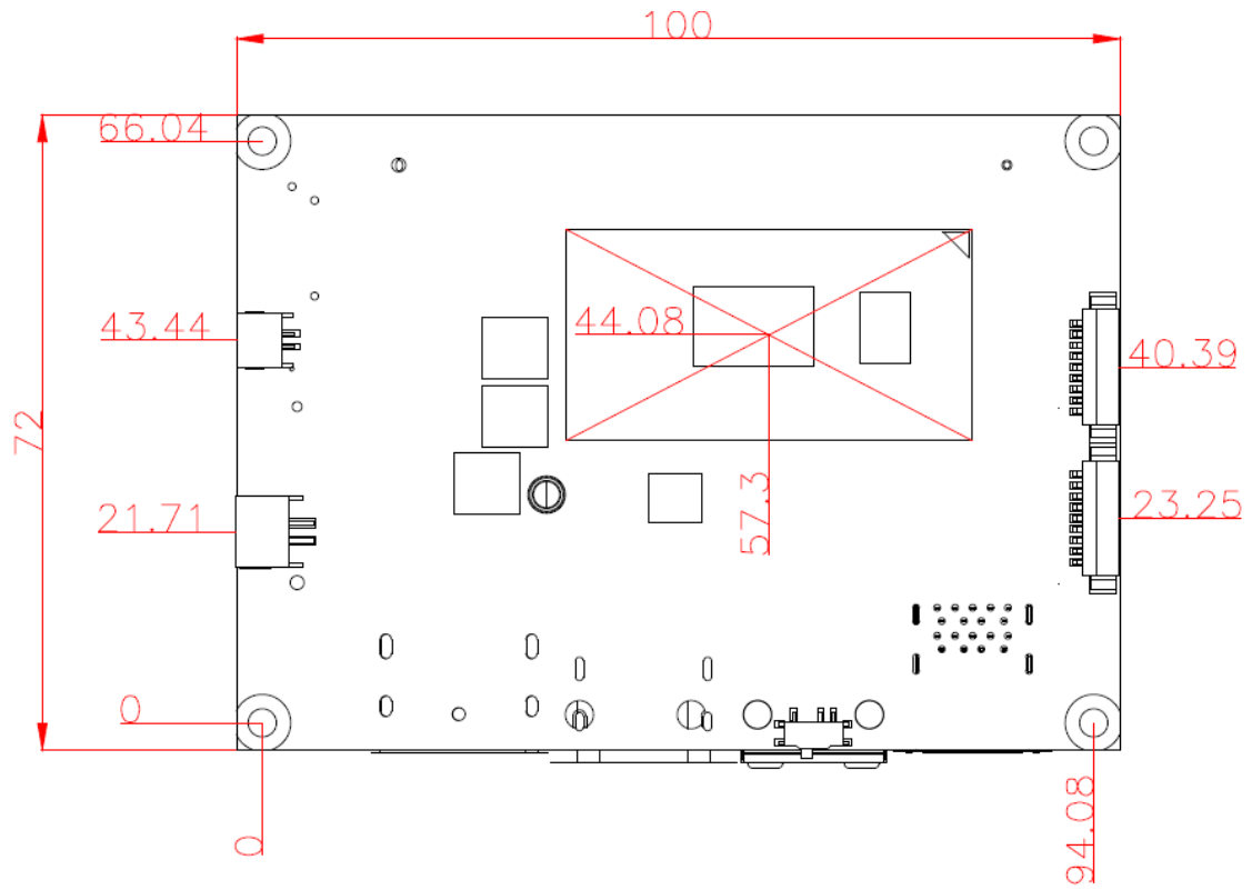
Bottom View
