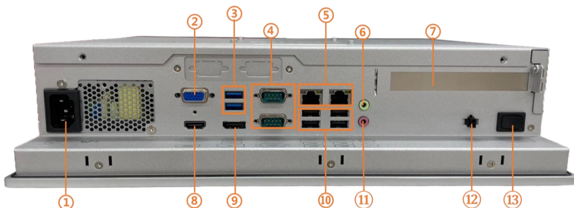
Figure 1-3 Side View of the P115-ADL-TRA
