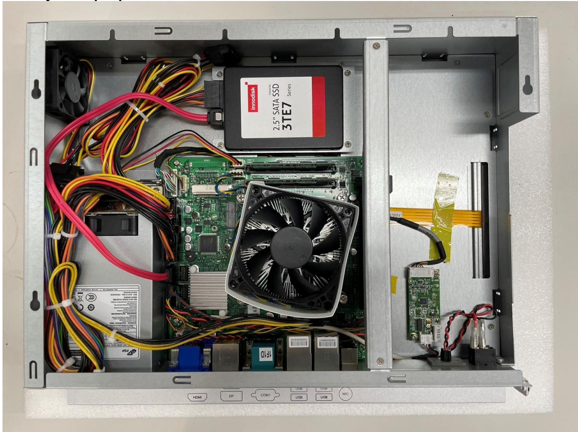
Figure 2-2 After Removing the back cover of the P115-ADL-TRA, install memory, storage and any other peripheral.
