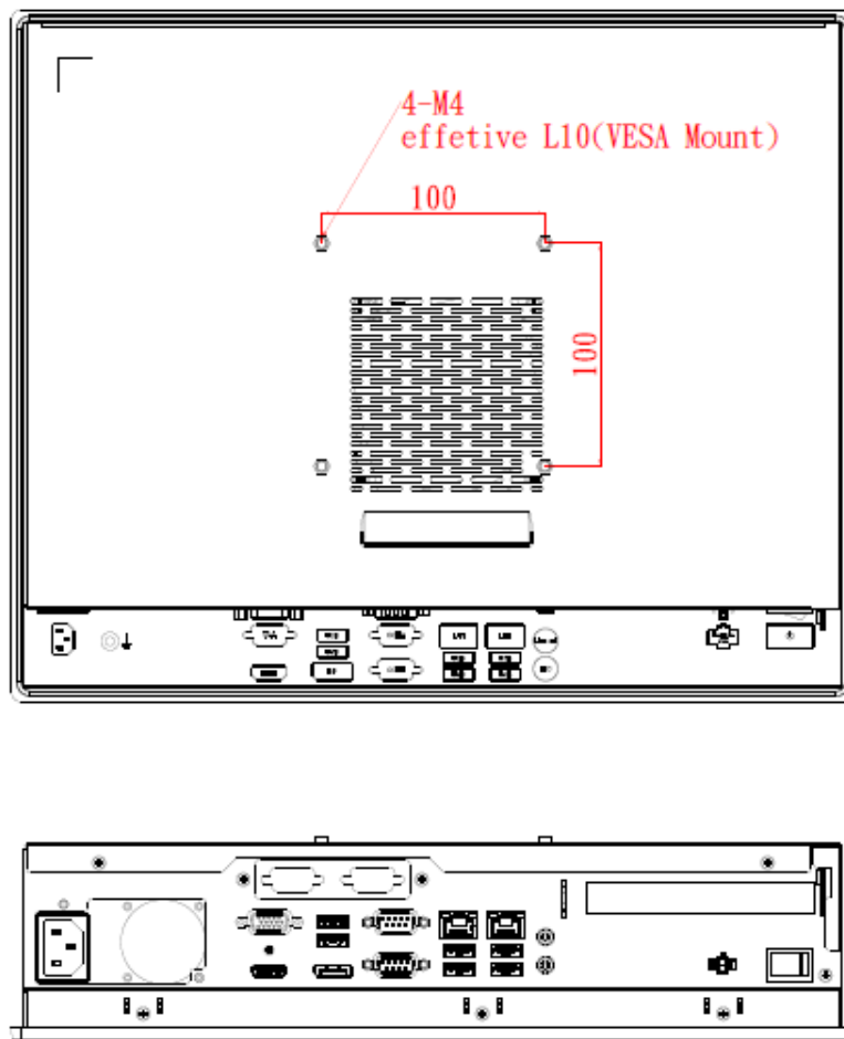
Diagram 1-2 Back outline of the P115-ADL-TRA
