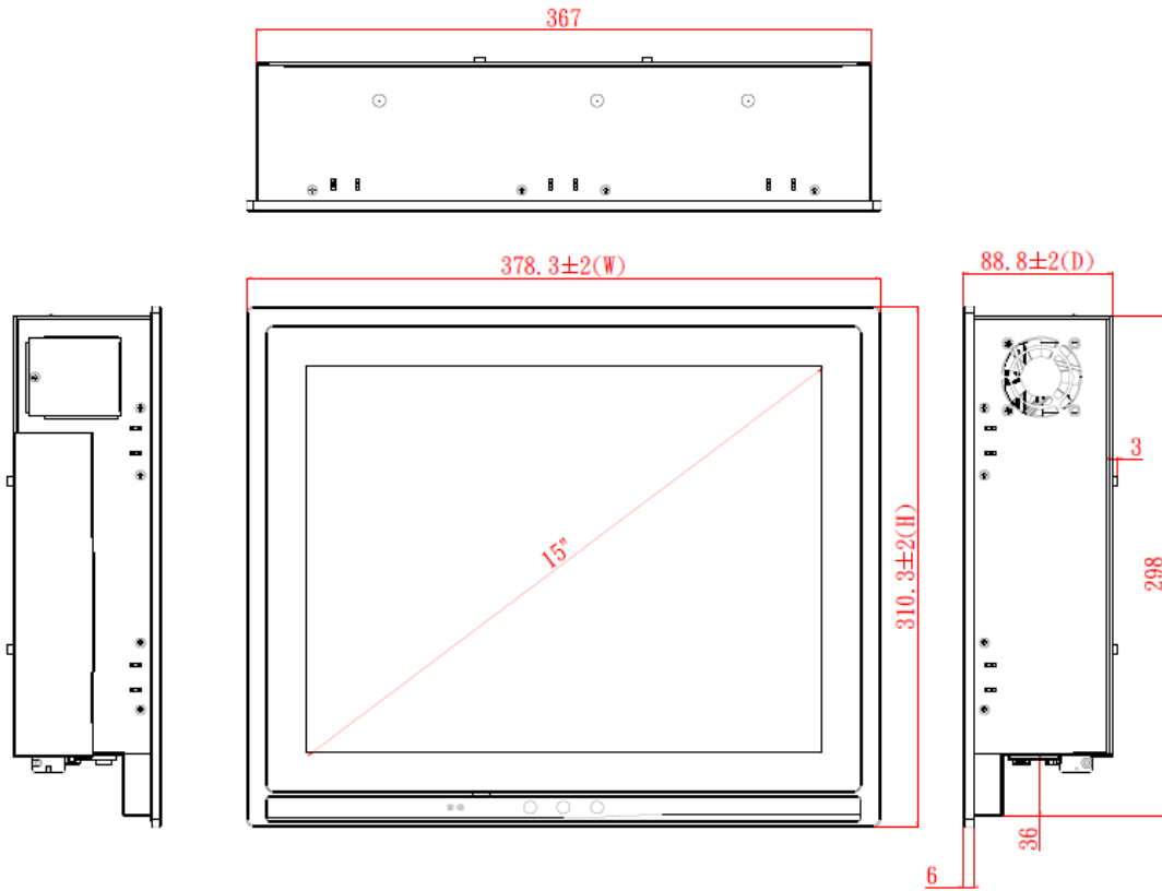
Diagram 1-1 Outlines of the P115-ADL-TRA
