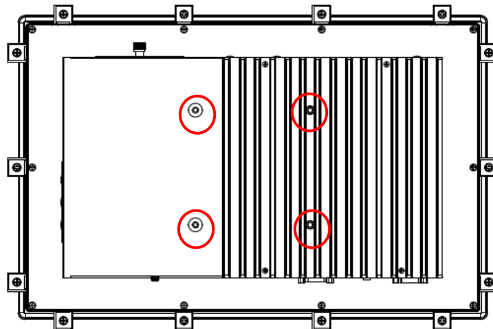
Diagram 2-2 VESA / desktop mount (back chassis)
