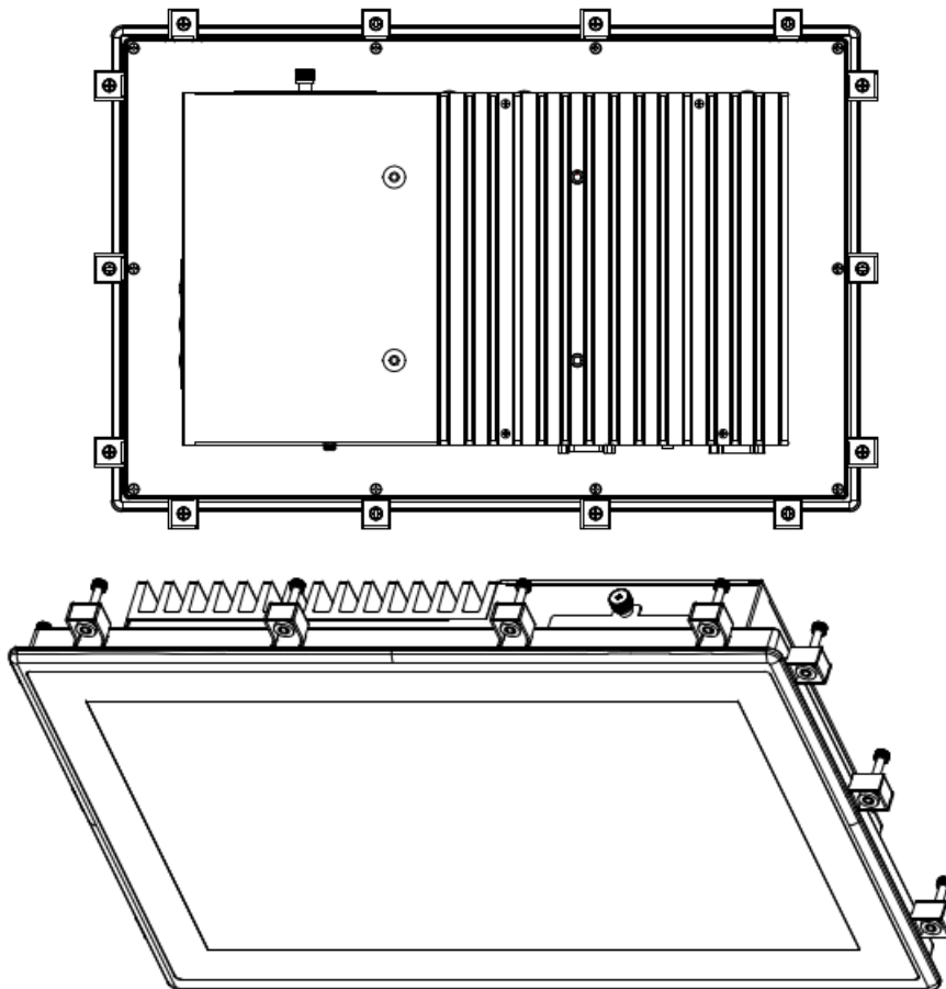
Diagram 2-1 Panel mount kit
