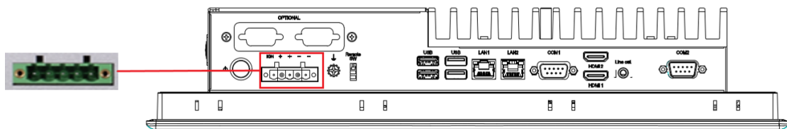
Figure 2-3: Power connector
