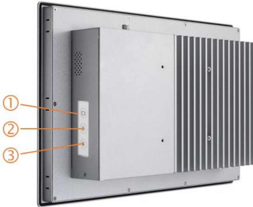
Figure 1-2 Side View of the GOT315B-ADL-WCD
