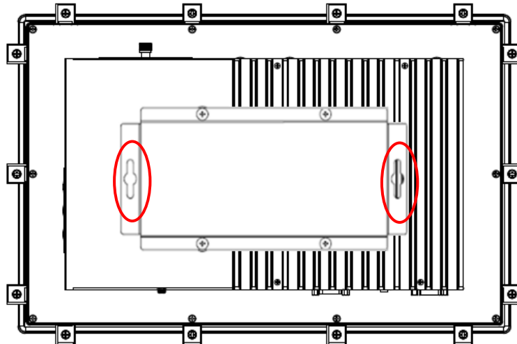
Diagram 2-3 Wall mount (back chassis)
