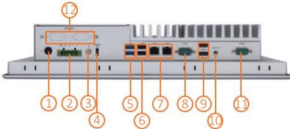
Figure 1-3 Side View of the GOT315B-ADL-WCD
