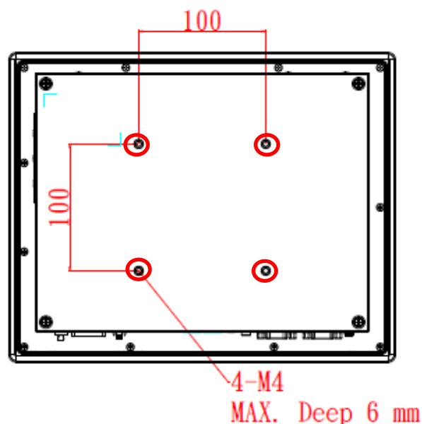
Figure 2-10: VESA mount screwing holes on the back chassis
