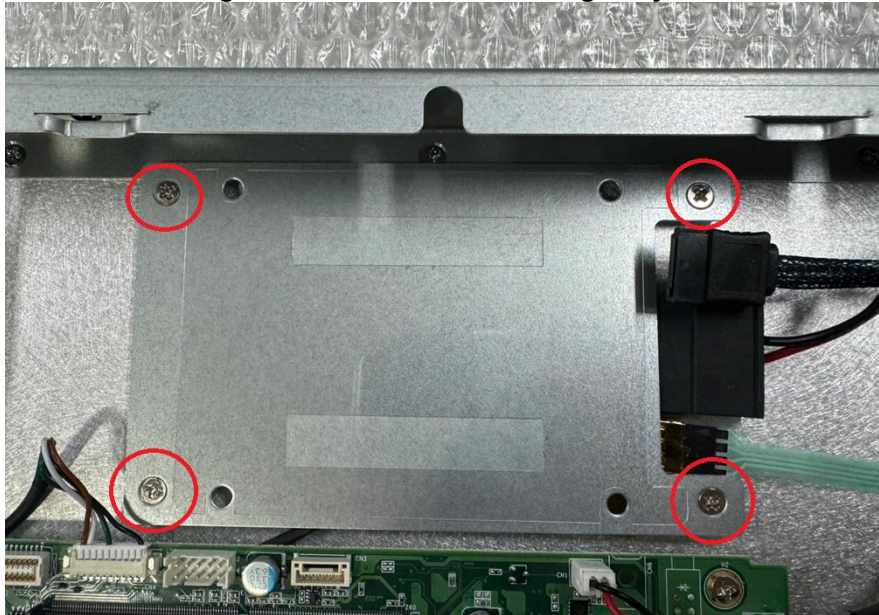
Figure 2-13: Remove the Storage tray
