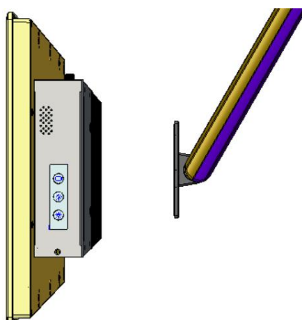
Figure 2-11: Assembling the VESA arm kit to the panel PC
