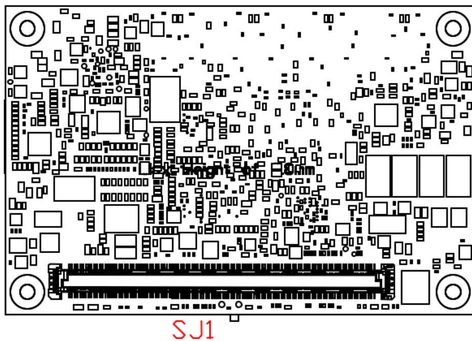
Bottom View
