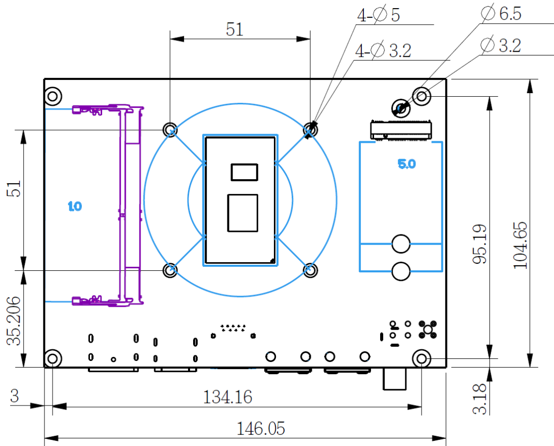
Bottom View
