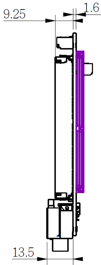
Side View
