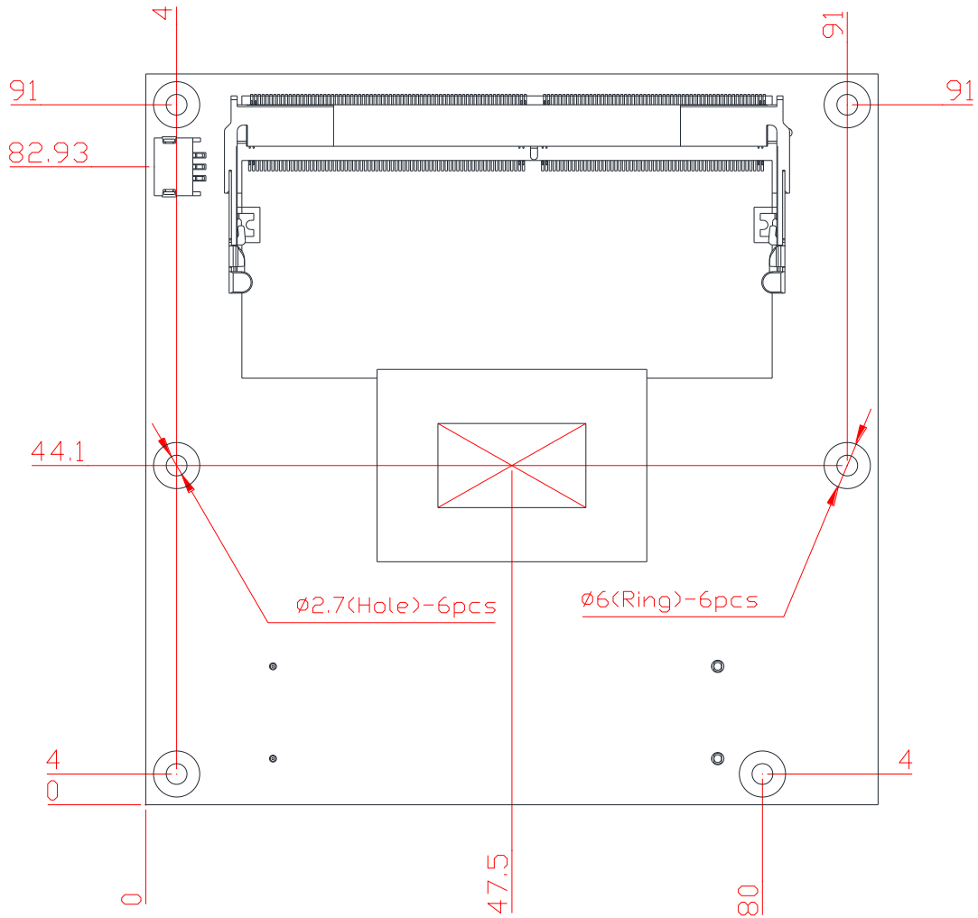
Top View
