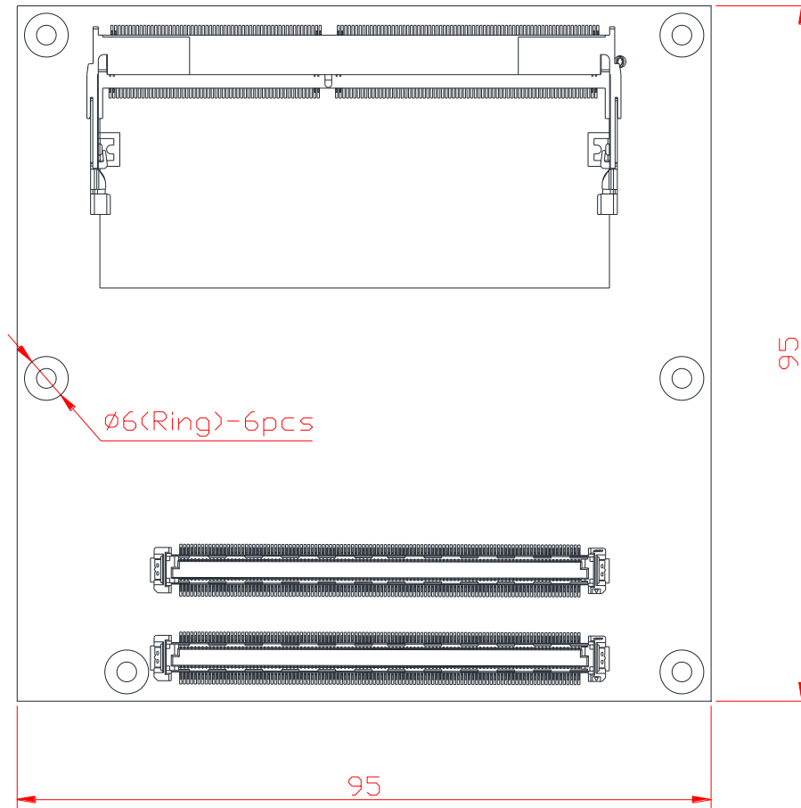
Bottom View
