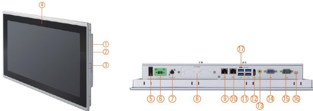
Figure 1-4: Bottom view of the GOT315A-ELK-WCD
