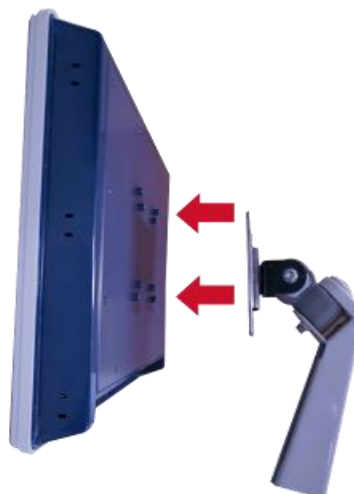
Figure 2-11: Assembling the VESA arm kit to the panel PC
