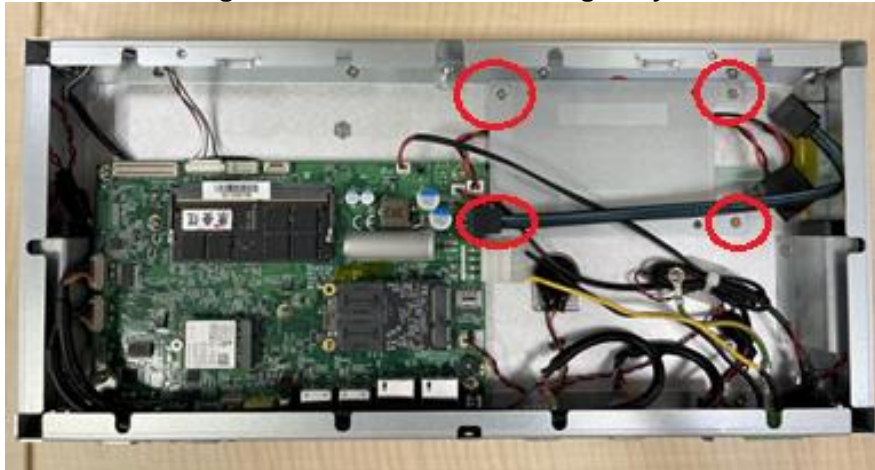
Figure 2-13: Remove the Storage tray
